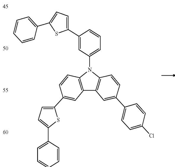
compound B
