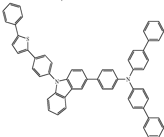
Formula 9
