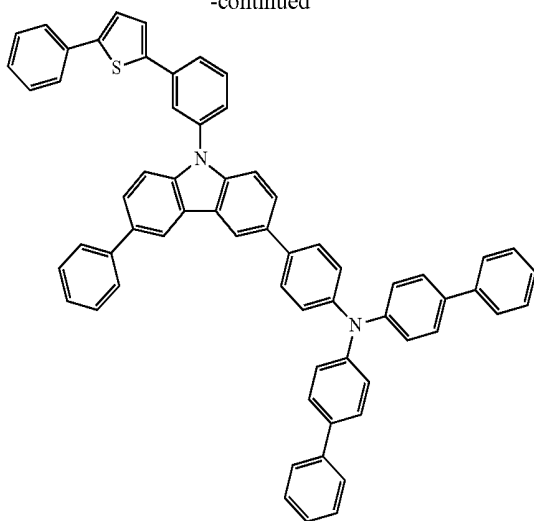
Formula 10
