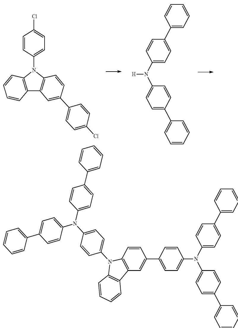
Formula 15
