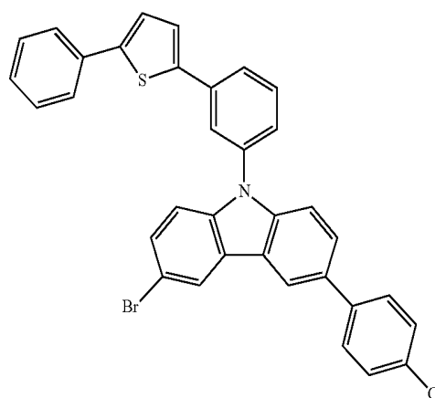
compound A
