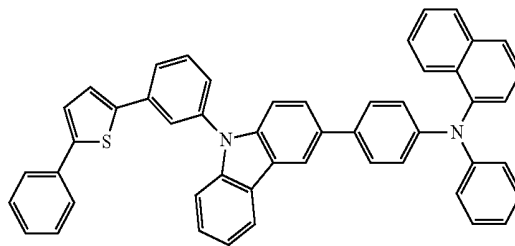
[Formula 7]
