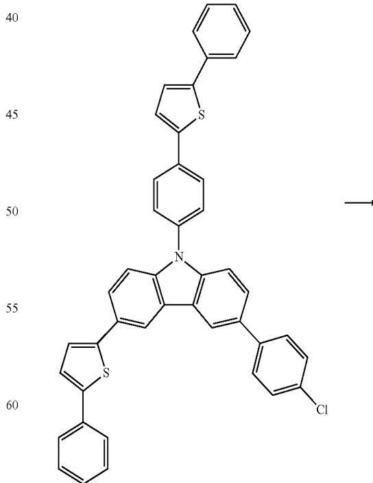
compound B
