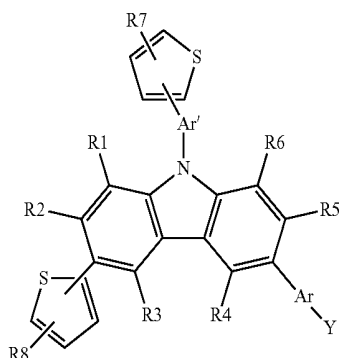
[Formula 2]
