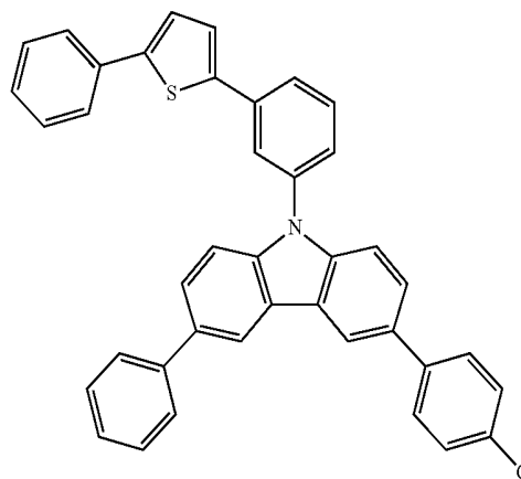
compound B
